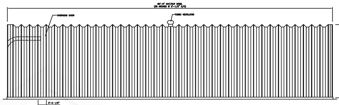
SIDE ELEVATION
